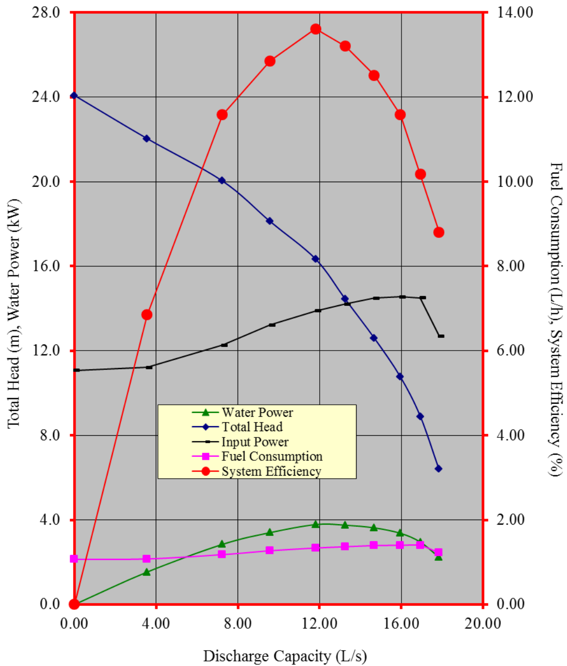
Figure 3. Performance characteristic curves of the OKAMA KDP3 self-priming centrifugal pumpset
